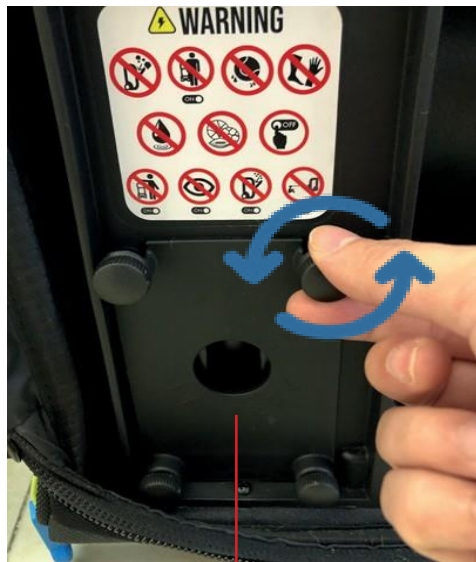
Battery Drawer
